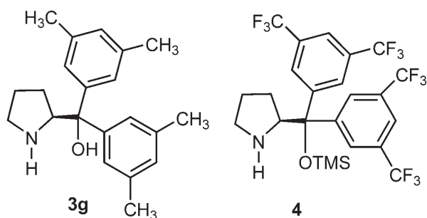
Figure 2. L-Proline-derived catalysts active in the epoxidation of enones and enals (TMS = trimethylsilyl).
