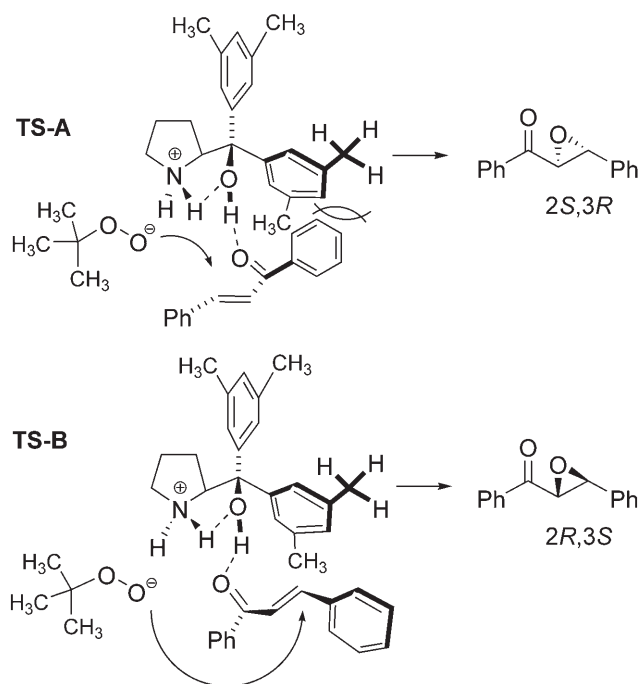
Scheme 3. Postulated transition states.
