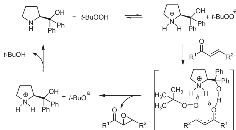
Scheme 2. Proposed catalytic cycle for the epoxidation.
